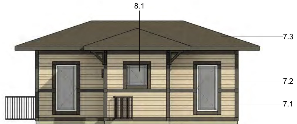
② Gazebo Front Elevation 1/8" = 1'-0"
